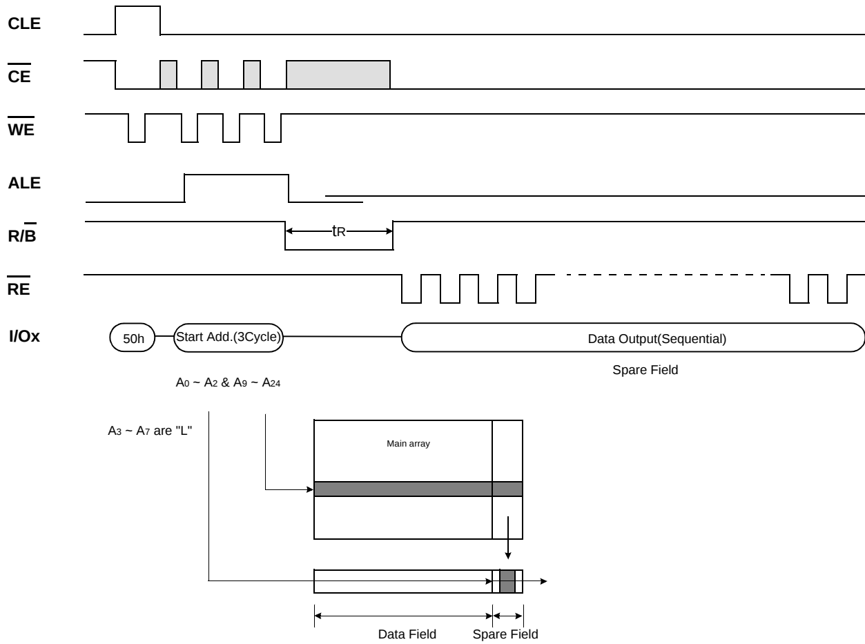
Figure 7. Read2 Operation
