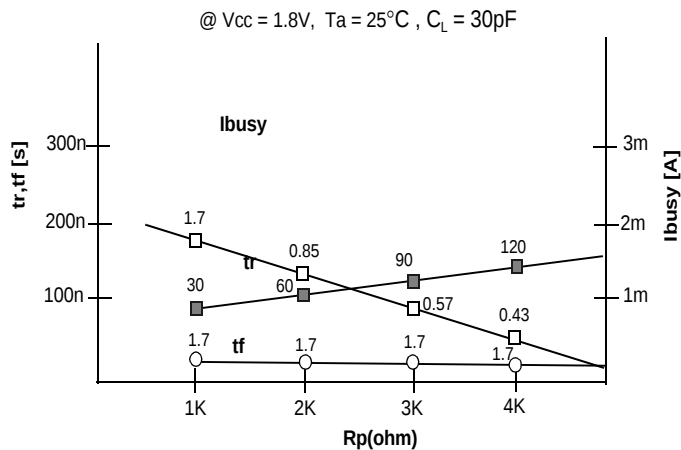
Figure 13. R_p vs t_r, t_f & R_p vs i_{\text{busy}}
