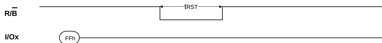
Figure 12. RESET Operation
