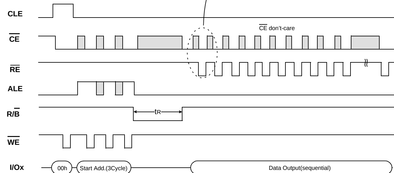
Figure 5. Read Operation with CE don't-care.
