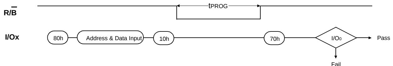
Figure 8. Program Operation
