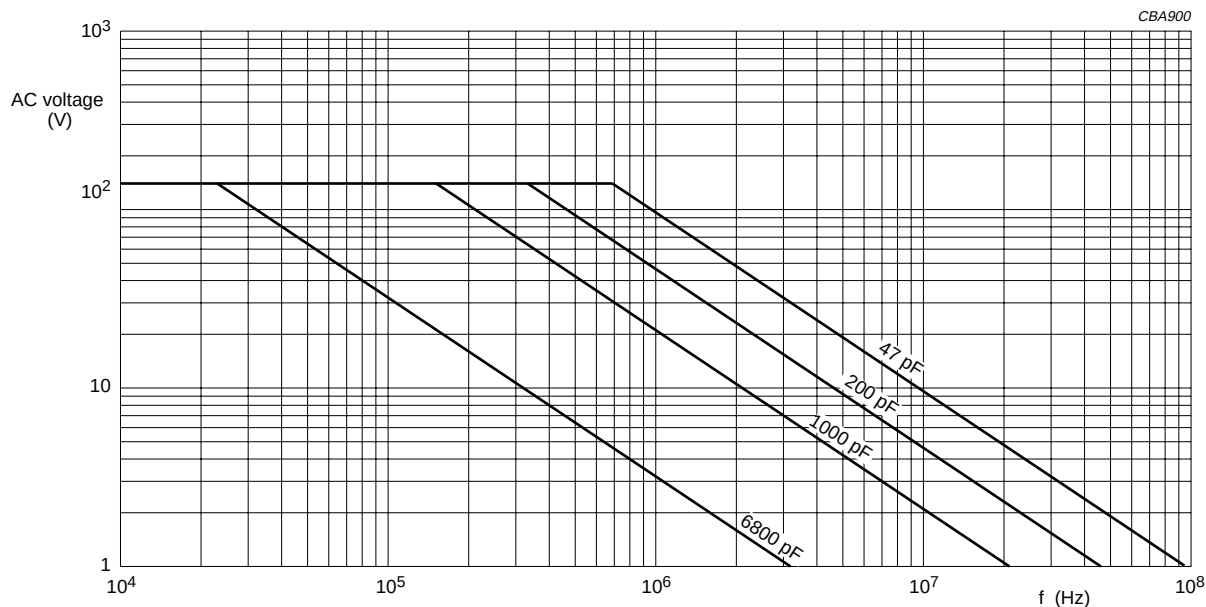
Fig.22 AC voltage (RMS value) as a function of frequency at 70\text{ }^{\circ}\text{C} < T_{amb} \leq 100\text{ }^{\circ}\text{C} for U_{Rdc} = 630\text{ V} .
