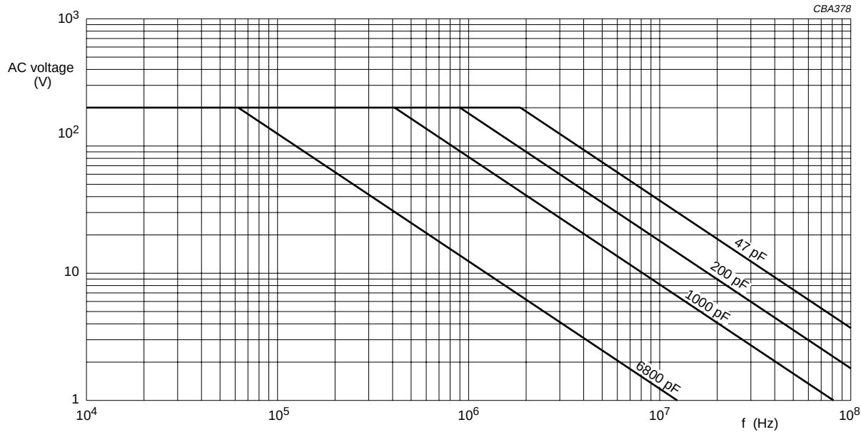
Fig.21 AC voltage (RMS value) as a function of frequency at T_{amb} \leq 70\text{ }^{\circ}\text{C} for U_{Rdc} = 630\text{ V} .
