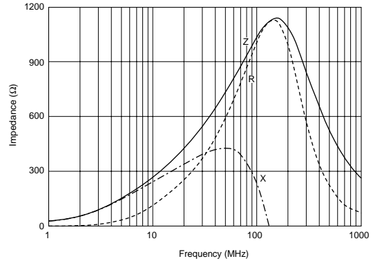
BLM18AG102SN1
