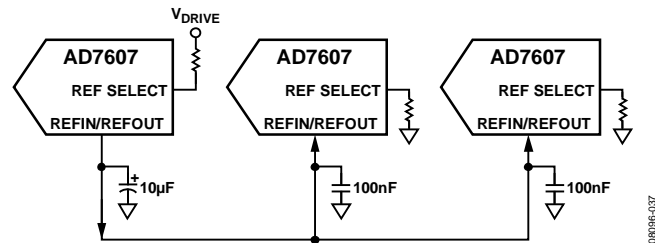
Figure 38. Internal Reference Driving Multiple AD7607 REF IN Pins.
