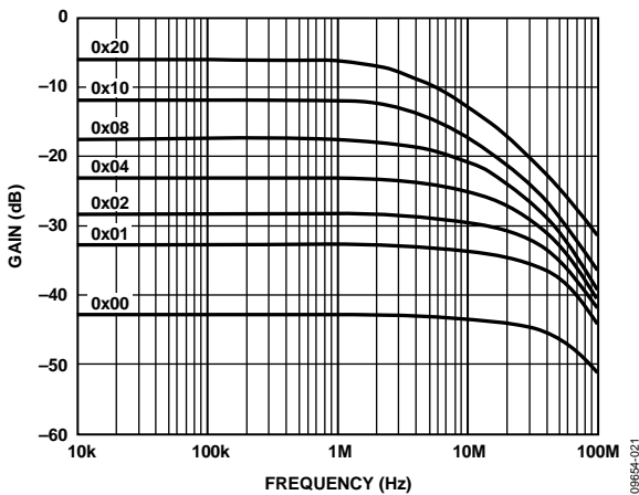
Figure 20. 5 kΩ Gain vs. Frequency vs. Code
