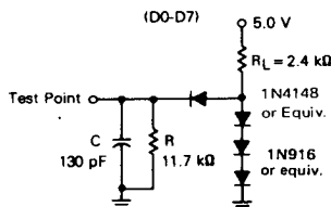
FIGURE 2 — BUS TIMING TEST LOADS
