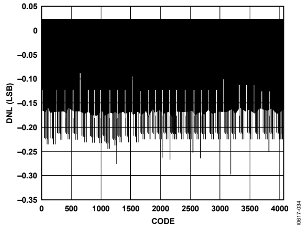
Figure 34. Typical DNL
