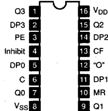
NTE4522B (BCD) 16-Lead DIP, See Diag. 249 NTE4526B (Binary) Programmable Divide-by-"N" 4-Bit Counter
