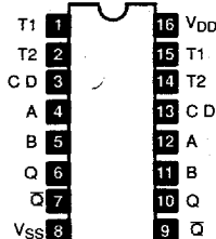
NTE4528B 16-Lead DIP, See Diag. 249 Dual Retriggerable/Resetable Monostable Multivibrator
