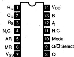
NTE4541B 14-Lead DIP, See Diag. 247 Programmable Timer
