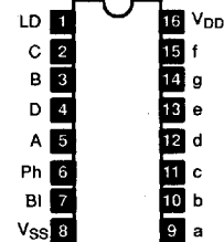
NTE4543B 16-Lead DIP, See Diag. 249 BCD-to-7-Segment Latch/Decoder/Driver for Liquid Crystals
