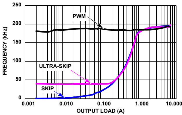
FIGURE 23. V_{OUT1} = 1.5V FREQUENCY vs LOAD
