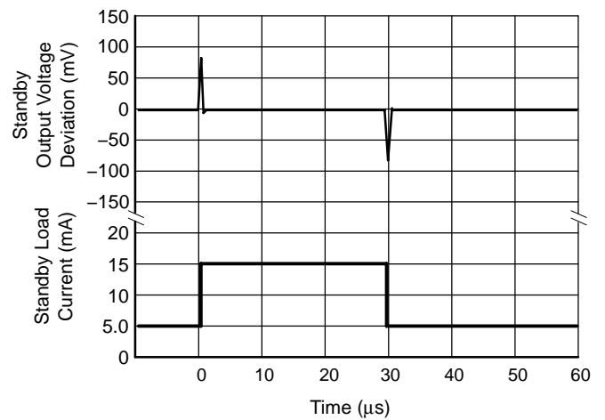
Figure 11. Load Transient Response ( V_{OUT2} )
