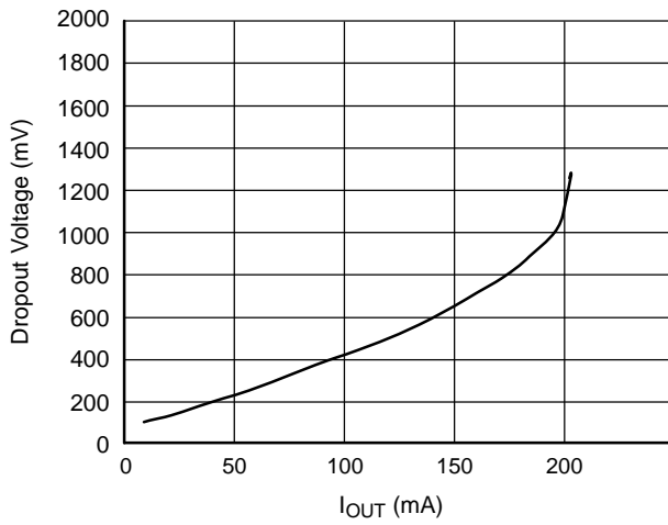
Figure 2. Dropout Voltage vs. I_{OUT}
