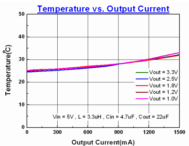
Figure 19. Temperature vs. Output Current
