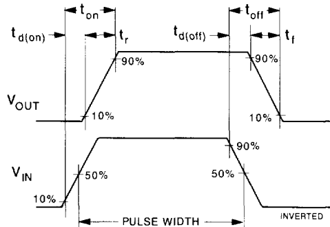
Figure 12. Switching Waveforms.
