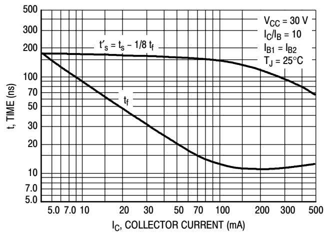
Figure 4. Turn-Off Time
