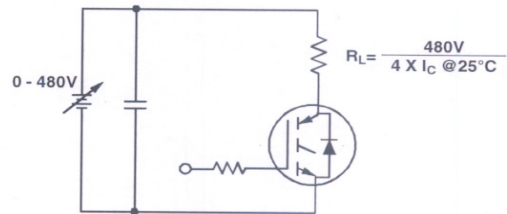
Figure 20. Pulsed Collector Current Test Circuit
