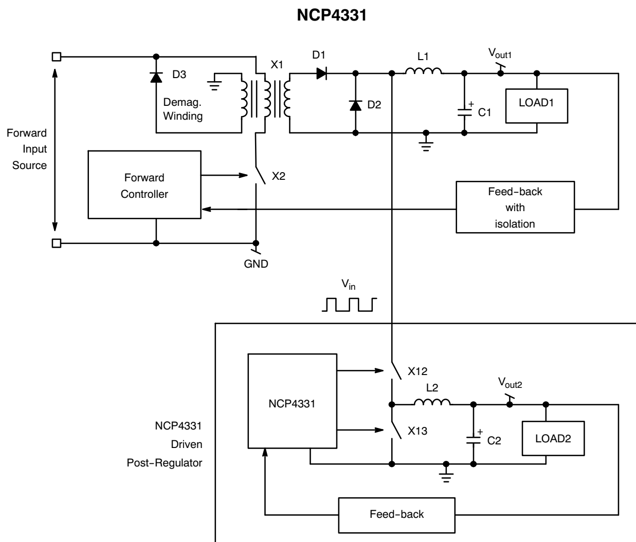
Figure 20. NCP4331 Post-Regulator Associated to a Forward Converter
