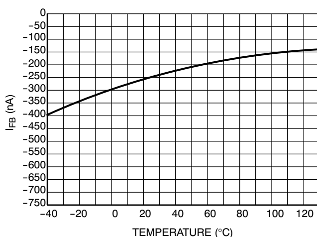
Figure 4. FB Pin Bias Current versus Temperature
