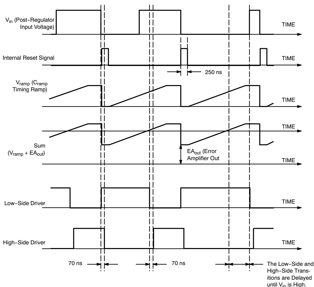
Figure 22. Timing Diagram
