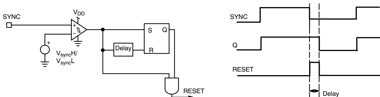
Figure 24. Synchronization Block
