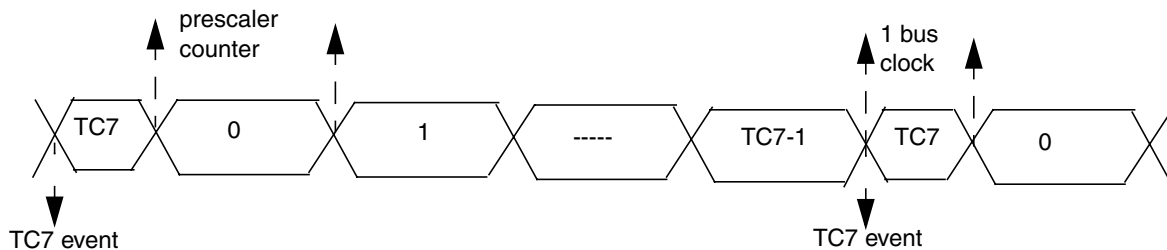
Figure 14-17. The TCNT cycle diagram under TCRE=1 condition
