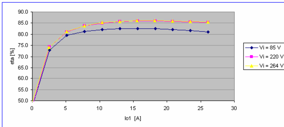
Figure 1. Efficiency vs. Output Load
