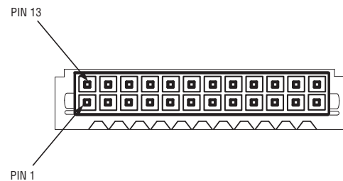
Connector: Molex (15-06-0241)
