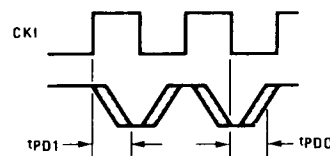
Figure 3B. CKO Output Timing
