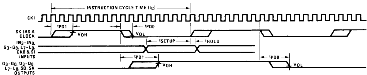
Figure 3. Input/Output Timing Diagrams (crystal divide by 16 mode)
