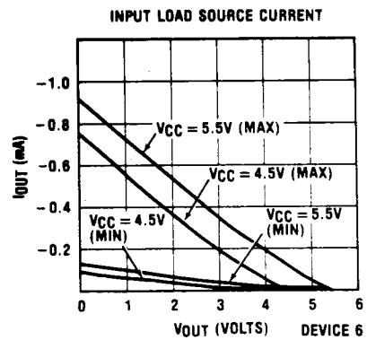
Figure 9c. ET9320/9321 Input/Output Characteristics
