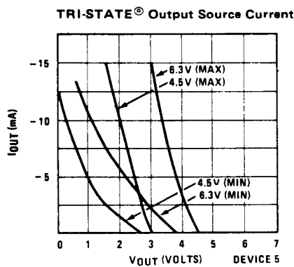
Figure 9b. ET9420/9421 Input/Output Characteristics
