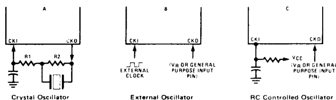
Crystal Oscillator
