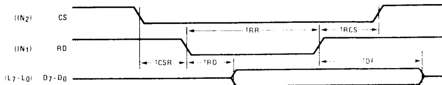
Figure 4. MICROBUS™ Read Operation Timing
