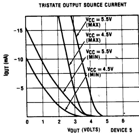
Figure 9c. ET9320/9321 Input/Output Characteristics
