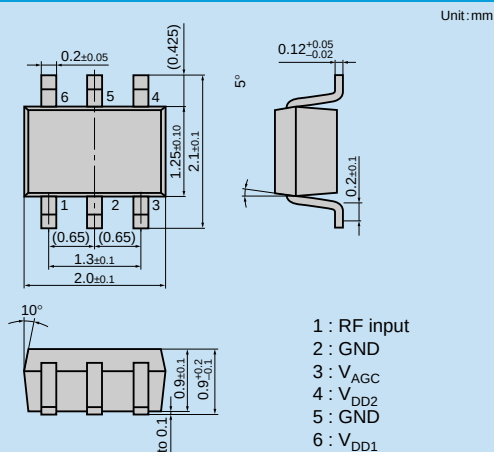
S-Mini Type-6-pin
