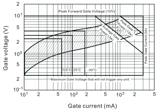
Fig.6 Gate characteristics
