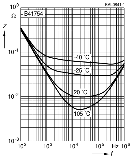
Impedance Z at different temperatures T Typical behavior for 3900 \mu F/63 V
