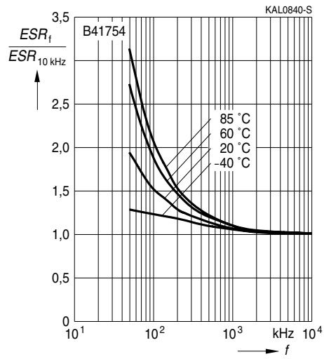
Frequency characteristics of ESR typical behavior
