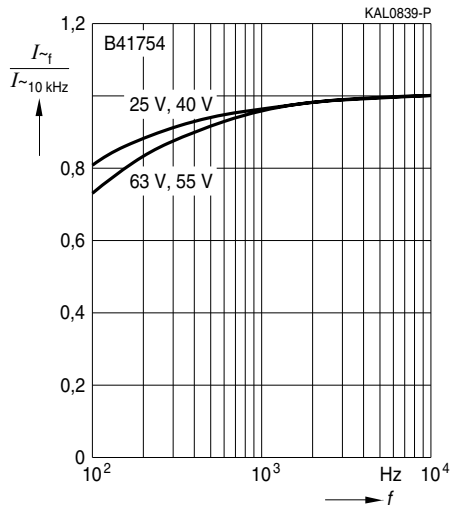
Frequency factor of permissible ripple current I_r versus frequency f
