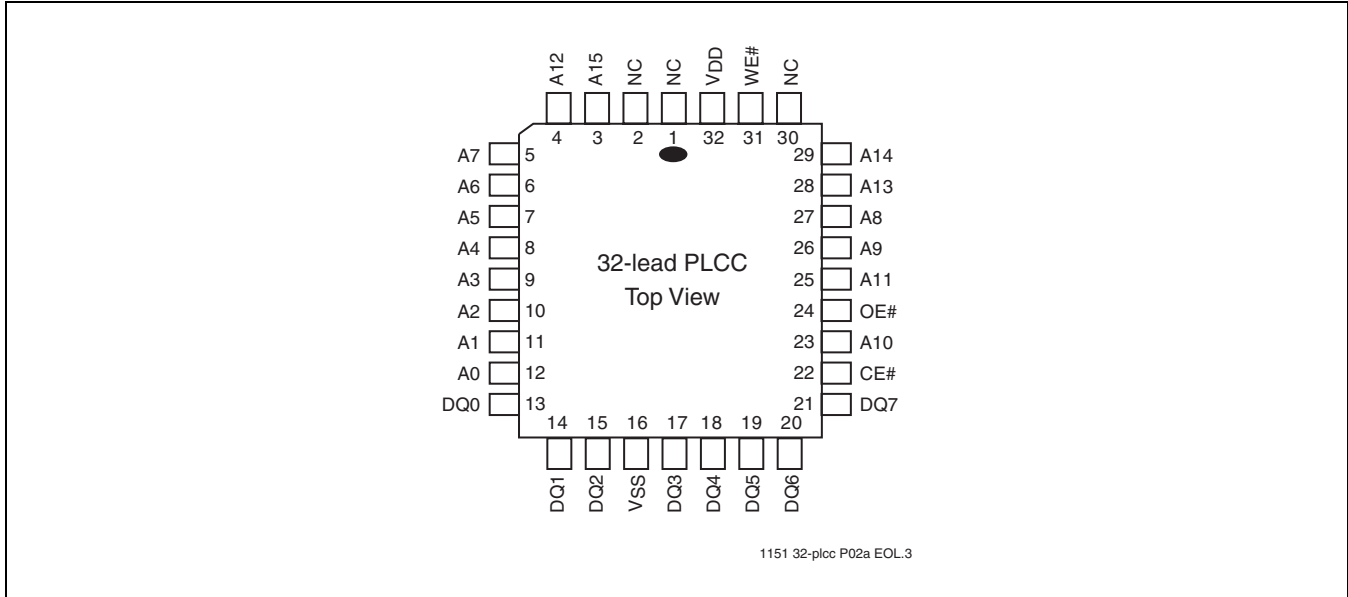
FIGURE 2: Pin Assignments for 32-lead PLCC
