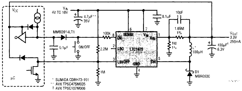
Figure 17. LTC1475 Regulator with 1-Button Toggle On/Off
