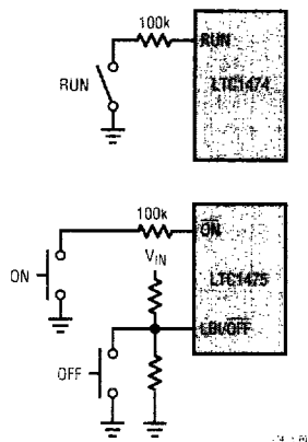
Figure 7. Simplified Implementation of LTC1474 and LTC1475 On/Off
