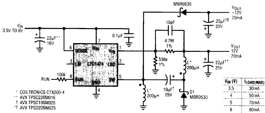
Figure 12. 5V to ±12V Regulator
