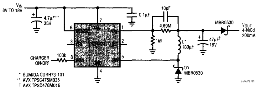
Figure 15. 4-NiCd Battery Charger
