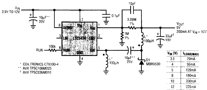
Figure 13. 5V Buck-Boost Converter
