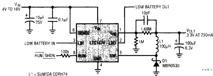
Figure 1. High Efficiency Step-Down Converter
