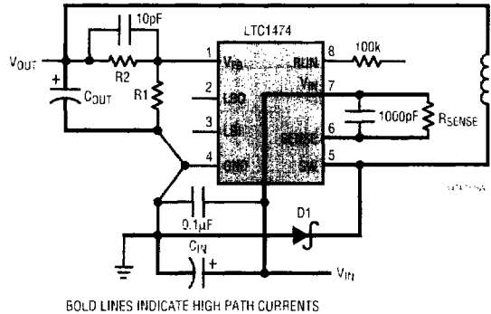
Figure 9. LTC1474/LTC1475 Layout Diagram (See Board Layout Checklist)
