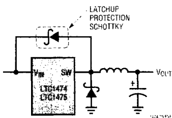
Figure 8. Preventing Absolute Maximum Ratings from Being Exceeded
