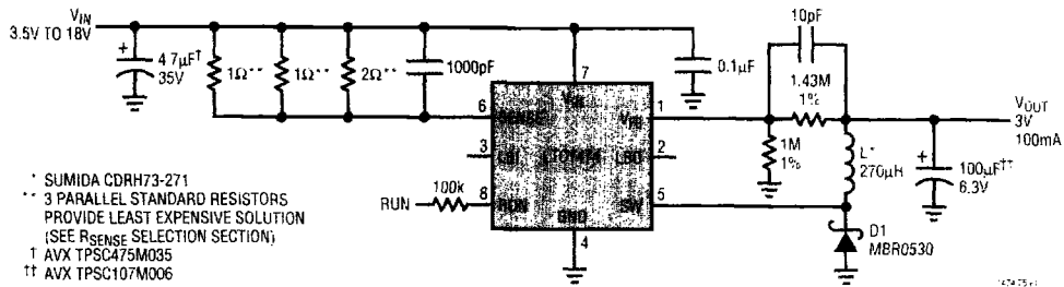
Figure 10. High Efficiency 3V/100mA Regulator
