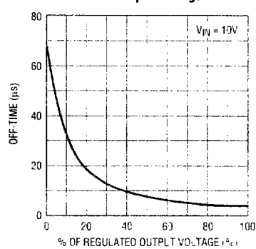
Off-Time vs Output Voltage
