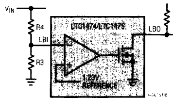
Figure 5. Low Battery Comparator
