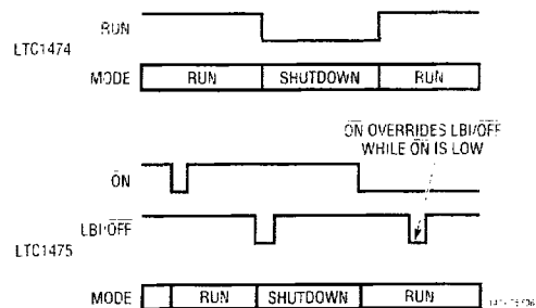
Figure 6. Comparison of LTC1474 and LTC1475 Run/Shutdown Operation
