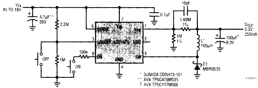
Figure 16. Pushbutton On/Off 3.3V/250mA Regulator
