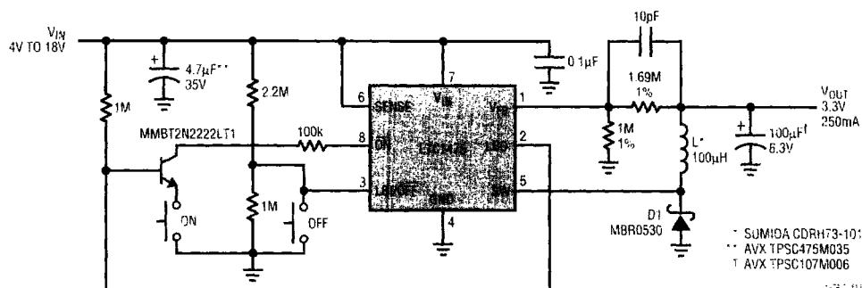
Figure 18. Pushbutton On/Off with Low Battery Lockout
