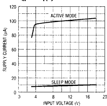
V_{IN} DC Supply Current
