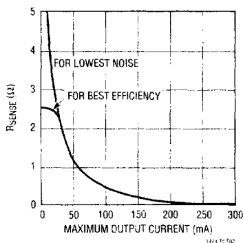
Figure 2. R_{SENSE} Selection
