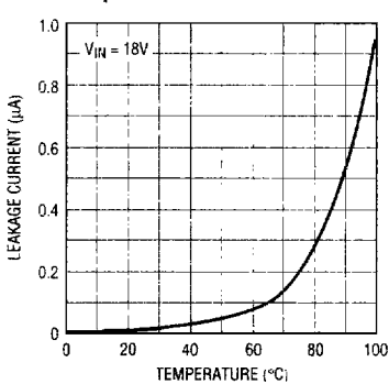
Switch Leakage Current vs Temperature
