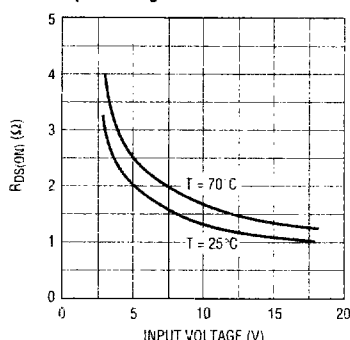
Switch Resistance vs Input Voltage
