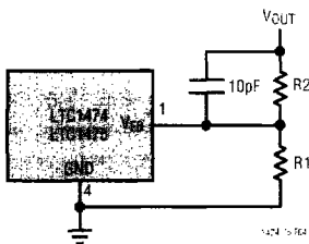
Figure 4. LTC1474/LTC1475 Adjustable Configuration
