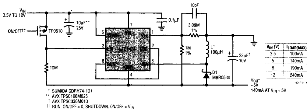
Figure 14. Positive-to-Negative (-5V) Converter
