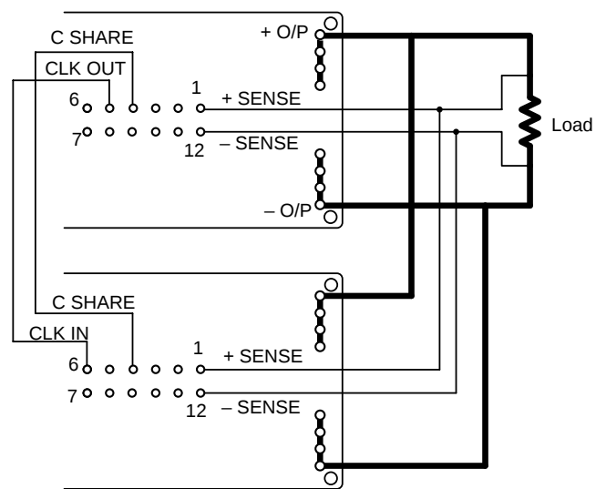
Parallel Connections
