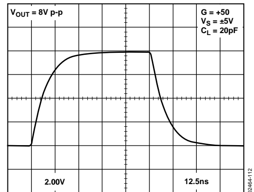
Figure 111. AD8129 Transient Response, V_{OUT} = 8\text{ V p-p}, G = +50, V_S = \pm 5\text{ V}
