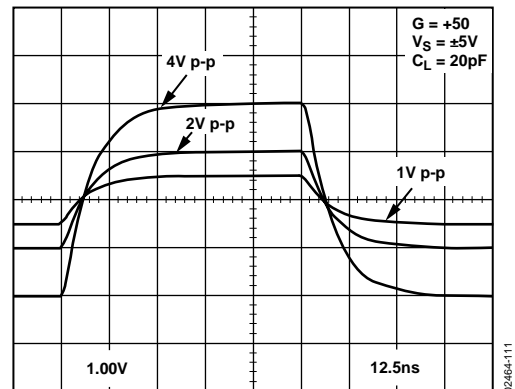
Figure 110. AD8129 Transient Response vs. Output Amplitude, V_{OUT} = 1\text{ V p-p}, 2\text{ V p-p}, 4\text{ V p-p}
