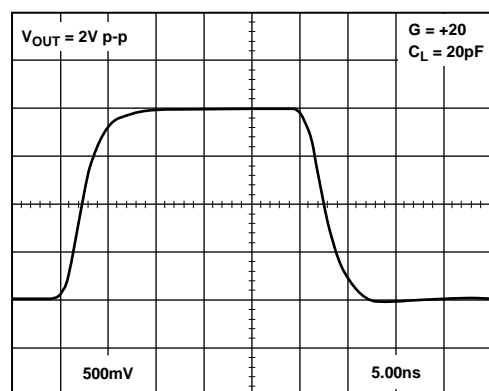
Figure 105. AD8129 Transient Response, V_{OUT} = 2\text{ V p-p} , V_S = \pm 5\text{ V}
