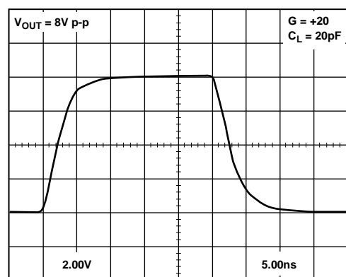
Figure 106. AD8129 Transient Response, V_{OUT} = 8\text{ V p-p} , V_S = \pm 5\text{ V}
