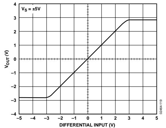
Figure 118. AD8130 Differential Input Clipping Level
