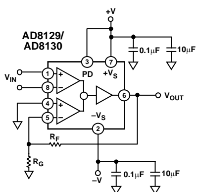
Figure 132. Basic Gain Circuit: V_{OUT} = V_{IN} (1 + R_F/R_G)
