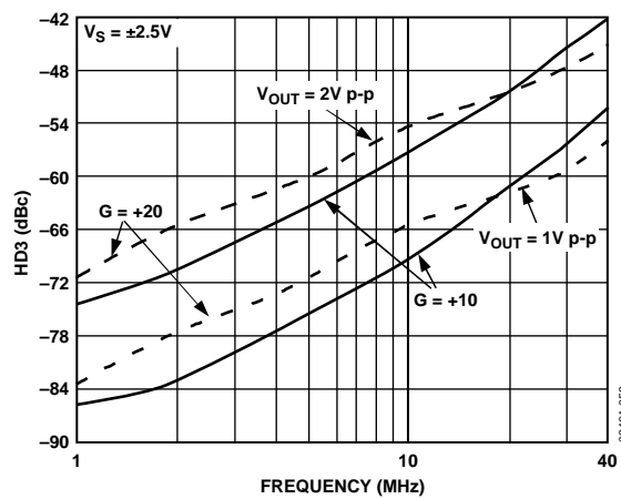
Figure 57. AD8129 Third Harmonic Distortion vs. Frequency
