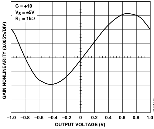
Figure 119. AD8129 Gain Nonlinearity, V_{OUT} = 2V p-p
