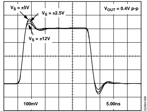
Figure 98. AD8129 Transient Response vs. Supply, V_{OUT} = 0.4 \text{ V p-p}
