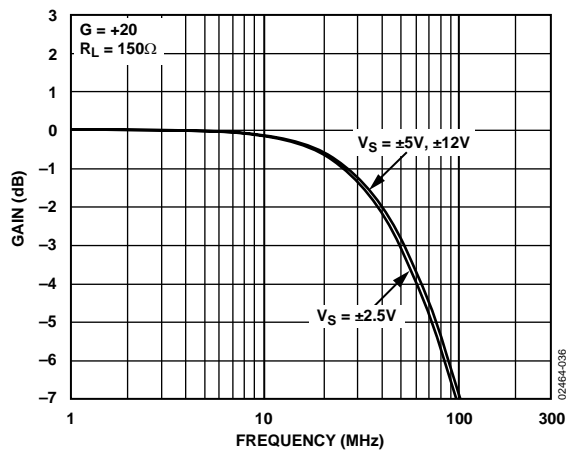
Figure 35. AD8129 Frequency Response vs. Supply, G = +20 , R_L = 150\ \Omega
