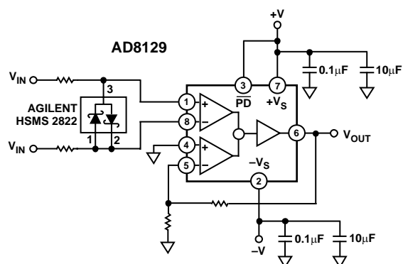
Figure 146. Schottky Diodes Across the Inputs Limits the Input Differential Voltage
