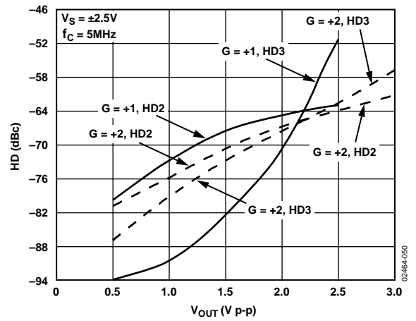
Figure 49. AD8130 Harmonic Distortion vs. Output Voltage
