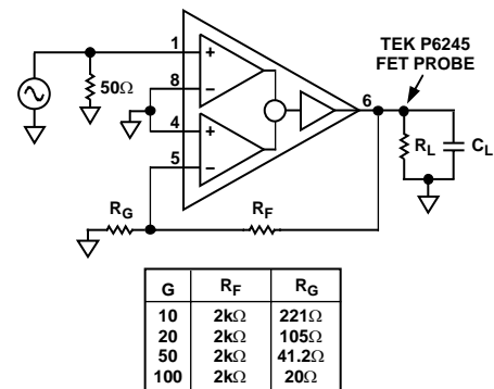
Figure 40. AD8129 Basic Frequency Response Test Circuit
