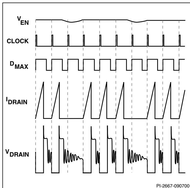
Figure 8. PeakSwitch Operation at Moderately Heavy Loading.
