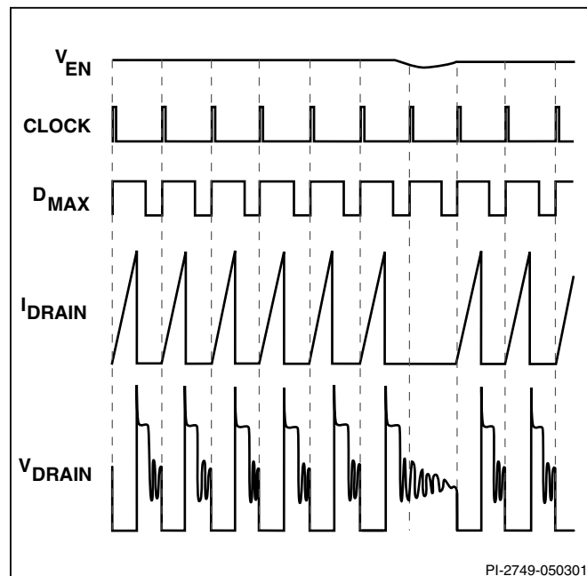
Figure 7. PeakSwitch Operation at Near Maximum Loading.
