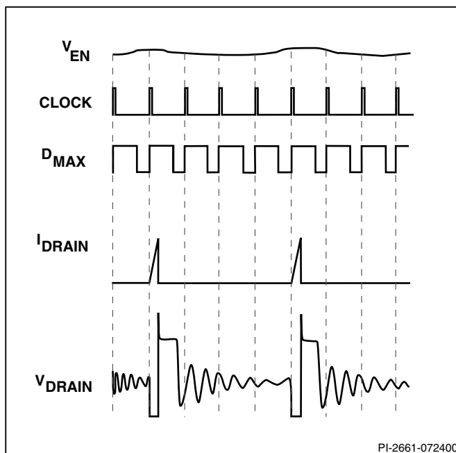
Figure 10. PeakSwitch Operation at Very Light Load.
