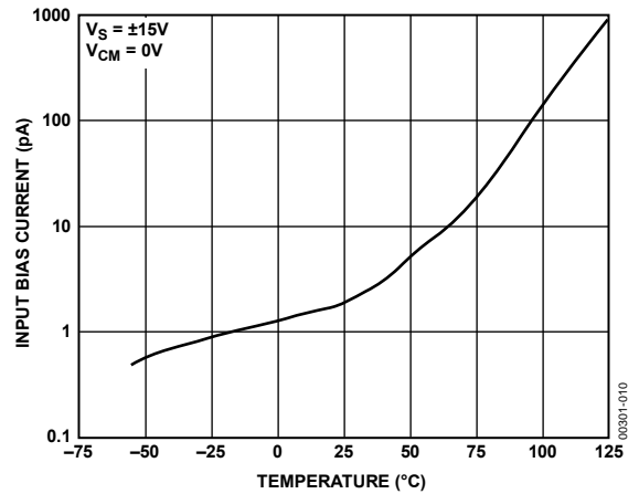
Figure 11. OP282 Input Bias Current vs. Temperature
