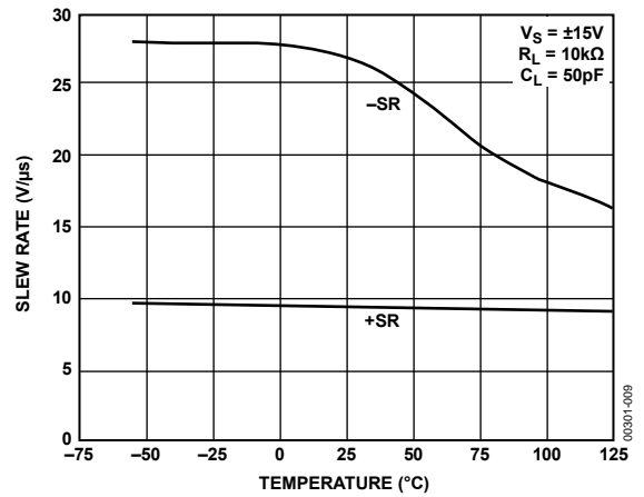
Figure 10. OP282 Slew Rate vs. Temperature
