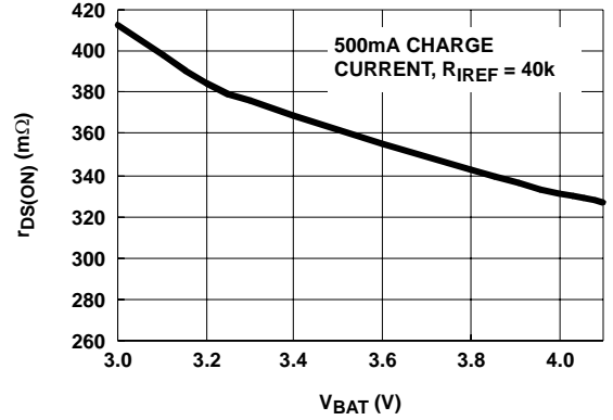
FIGURE 10. r_{DS(ON)} vs OUTPUT VOLTAGE USING CURRENT LIMITED ADAPTERS
