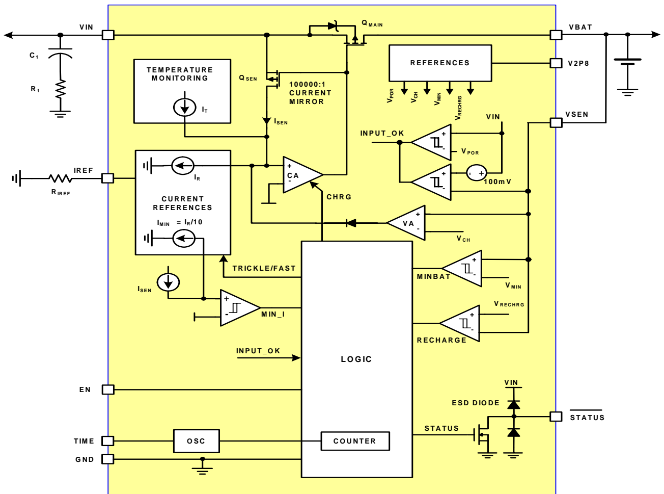
FIGURE 16. BLOCK DIAGRAM
