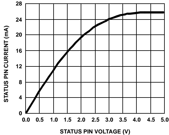
FIGURE 15. STATUS PIN VOLTAGE vs CURRENT WHEN THE OPEN-DRAIN MOSFET TURNS ON
