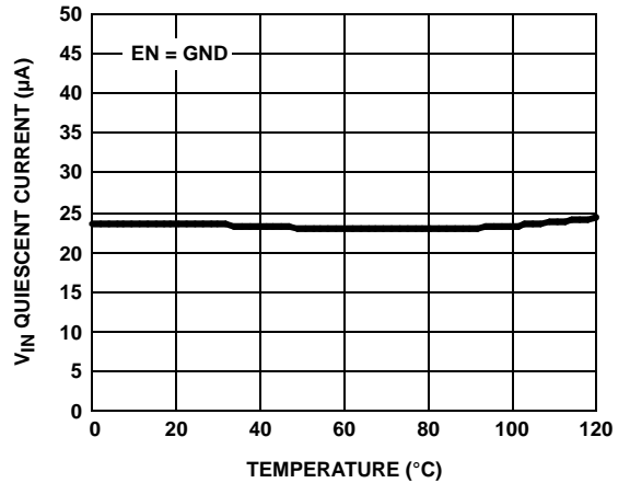
FIGURE 12. INPUT QUIESCENT CURRENT vs TEMPERATURE
