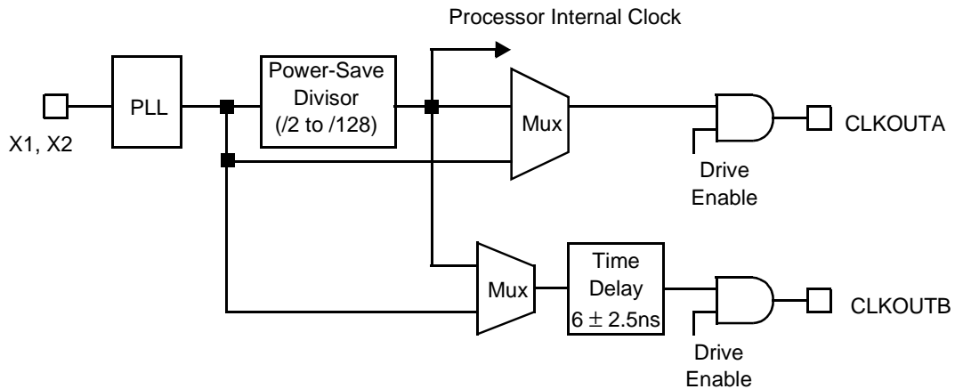
Figure 3-6 Clock Organization
