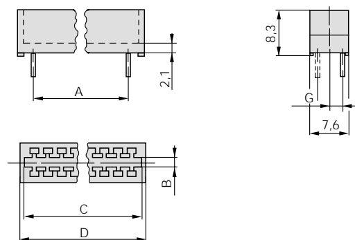
Without flange
