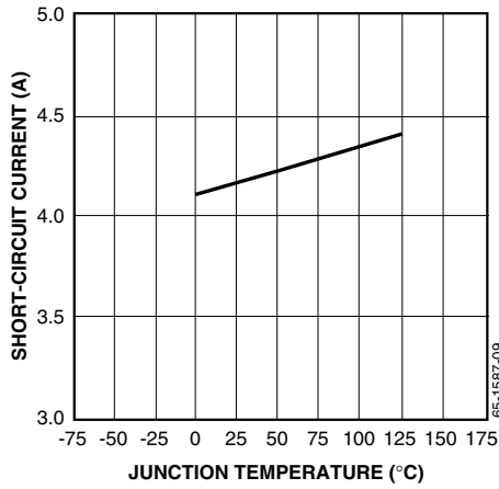
Figure 8. Short-Circuit Current vs. Temperature
