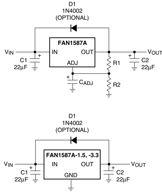
Figure 11. Optional Protection
