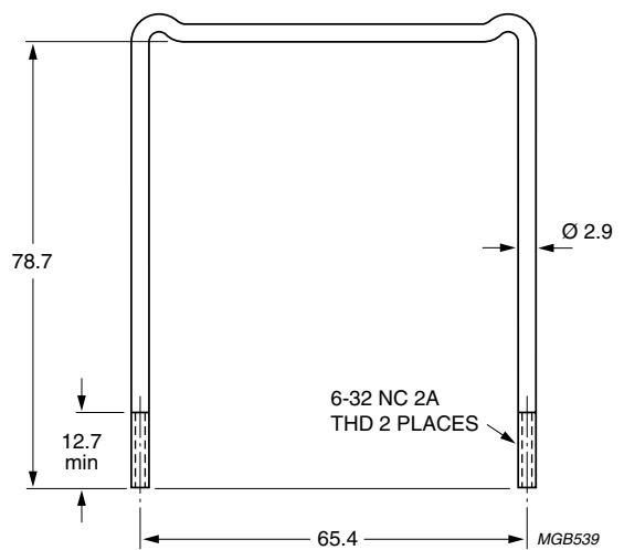
Fig.6 EC70 clamp.
