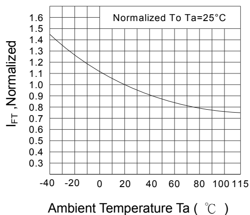
Trigger Current vs. Ambient Temperature
