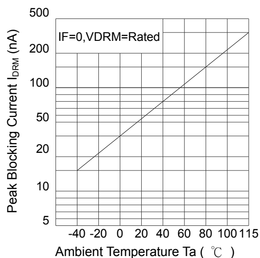
Leakage with LED off vs. Ambient Temperature
