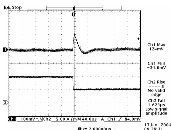
100% to 50% load step at V_{in}=5\text{ V} , V_o=2.5\text{ V}
