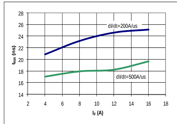
Figure 8. Typical t_{RR} vs I_F at T_J = 125^\circ\text{C}
