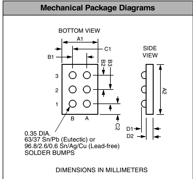
Package Dimensions for PACDN2404C 6-bump Chip Scale Package
