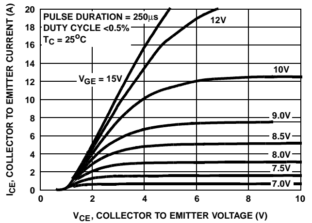
FIGURE 2. SATURATION CHARACTERISTICS
