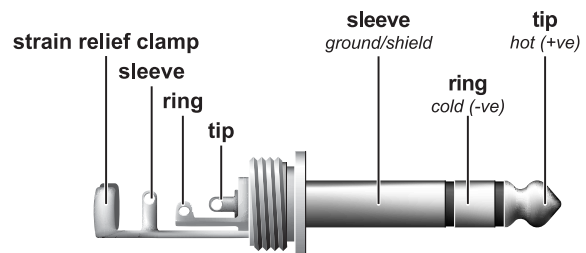
Fig. 4.4: 1/4" TRS connector
