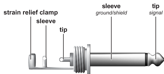
Fig. 4.3: 1/4" TS connector
