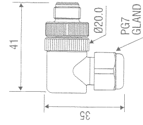
Micro-Change® (M12) Field Attachable Connectors - Male
