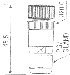
Micro-Change® (M12) Moulded Connectors - Female
