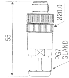
Micro-Change® (M12) Moulded Connectors - Male
