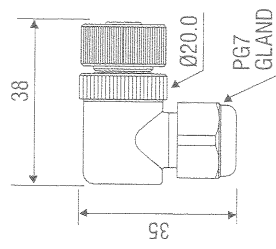
Micro-Change® (M12) Field Attachable Connectors - Female
