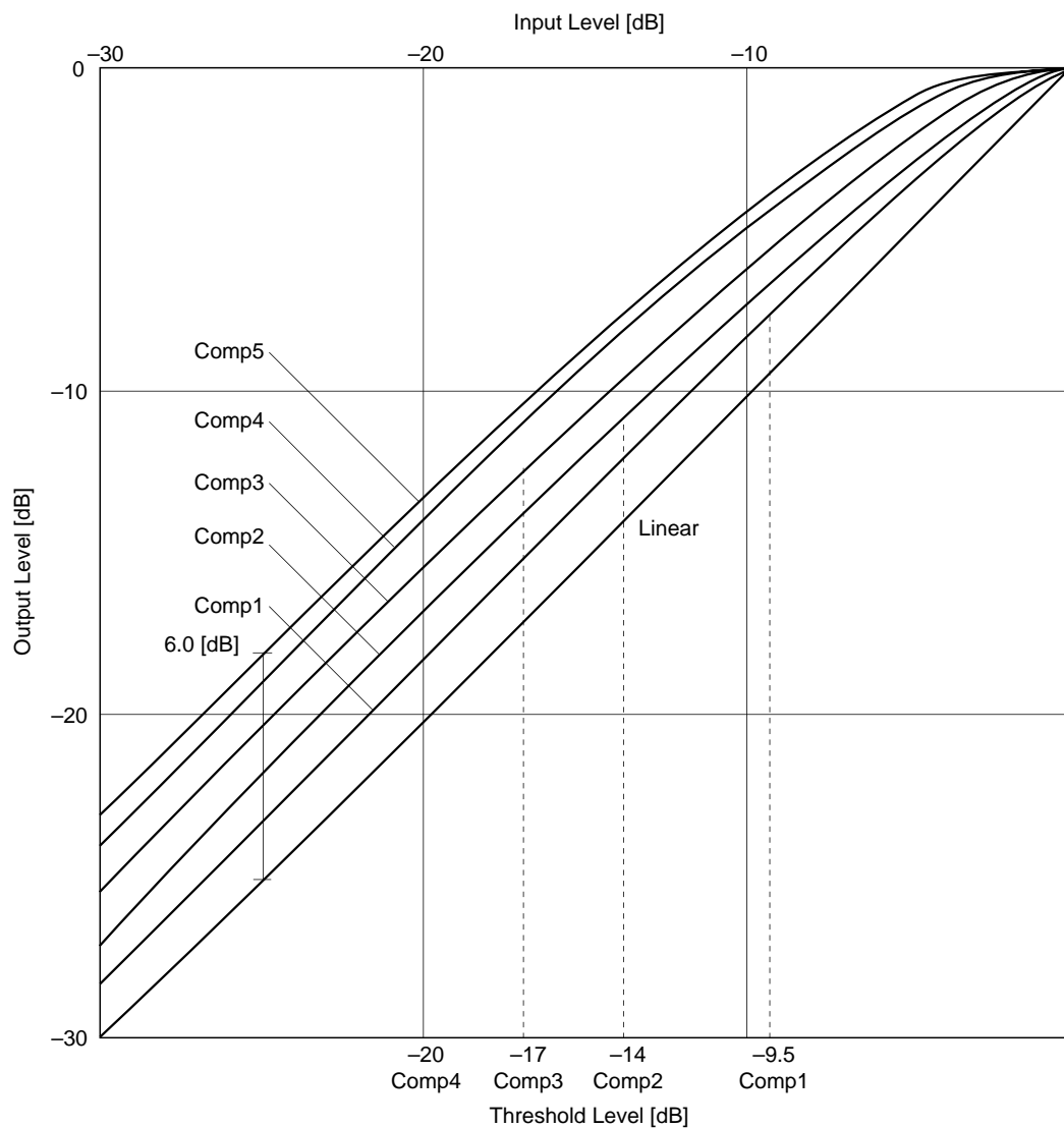
Fig. 8-4-2. Compressor I/O Characteristics
