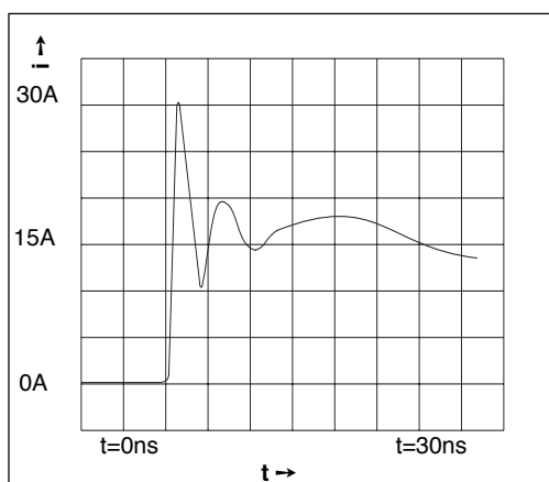
Figure 18. ESD Test Waveform for IEC1000-4-2
