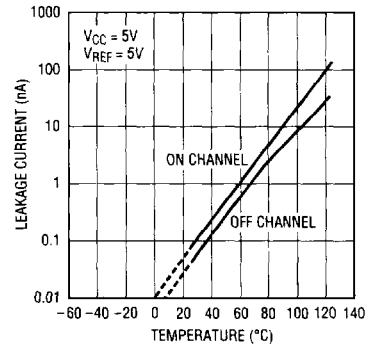
Input Channel Leakage Current vs Temperature
