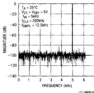
Figure 11. LTC1286 Non-Averaged, 4096 Point FFT Plot
