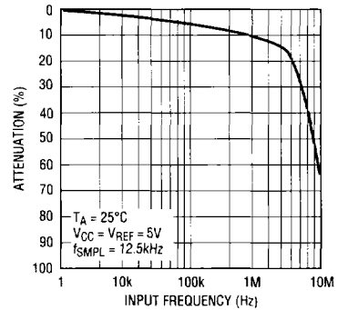
Attenuation vs Input Frequency
