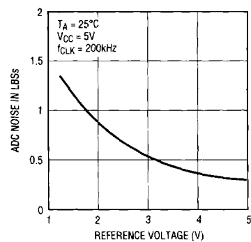
Peak-to-Peak ADC Noise vs Reference Voltage
