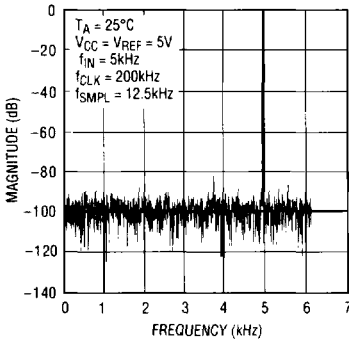
4096 Point FFT Plot
