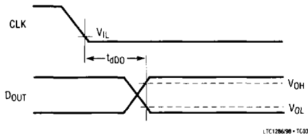
Voltage Waveforms for D_{OUT} Delay Times, t_{dDO}
