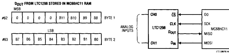
Hardware and Software Interface to the MC68HC11
