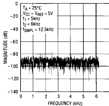
Intermodulation Distortion
