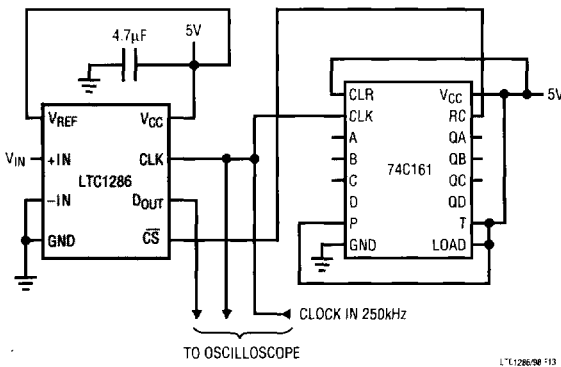
Figure 13. "Quick Look" Circuit for the LTC1286
