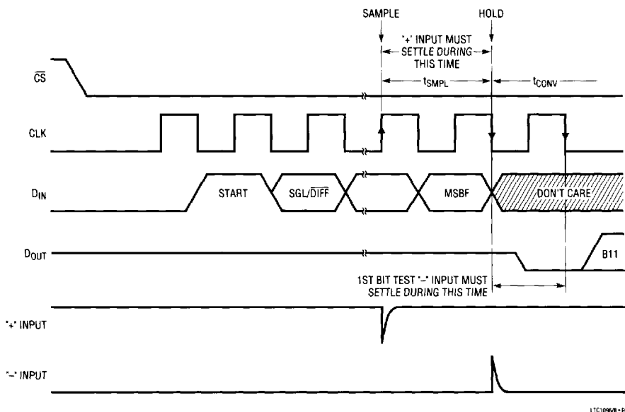
Figure 7. LTC1298 “+” and “-” Input Settling Windows
