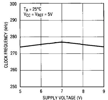
Maximum Clock Frequency vs Supply Voltage
