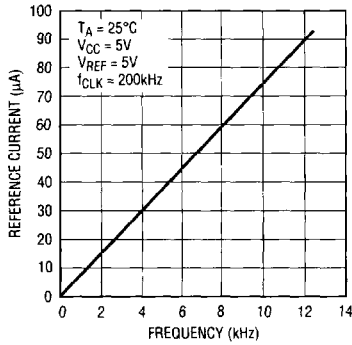
Reference Current vs Sample Rate (LTC1286)
