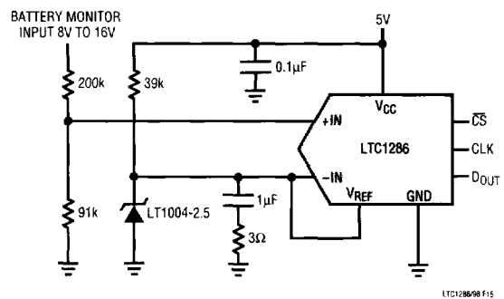
Figure 15. Micropower Battery Voltage Monitor
