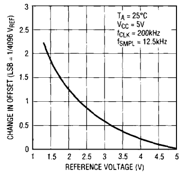
Change in Offset vs Reference Voltage
