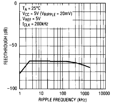
Power Supply Feedthrough vs Ripple Frequency
