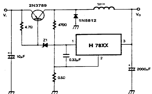
13、Switching Regulator
