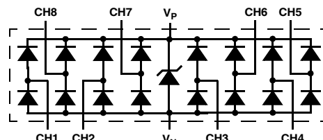
CM1293-08MS/MR
