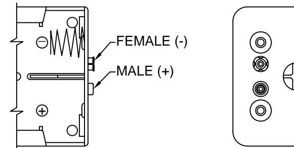
PDSN-14-1B SNAP TERMINAL
