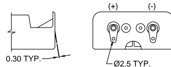
PDSN-14-1C SOLDER LUGS
