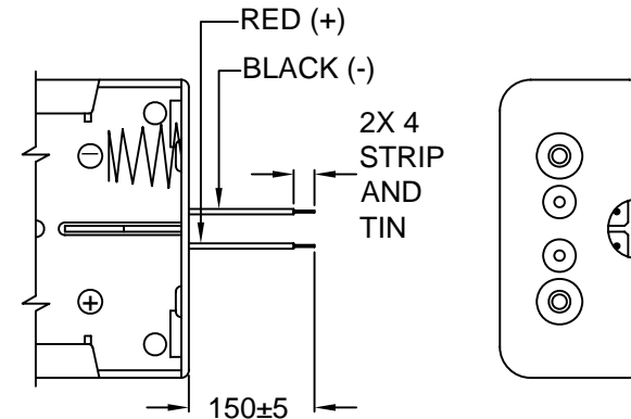
PDSN-14-1A WIRE LEADS
