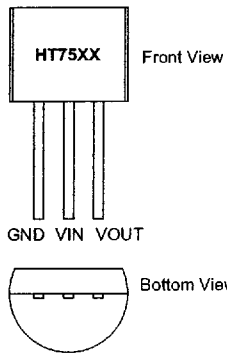
TO-92
