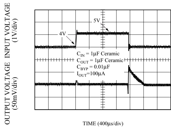
Fig. 6 Line Transient Response
