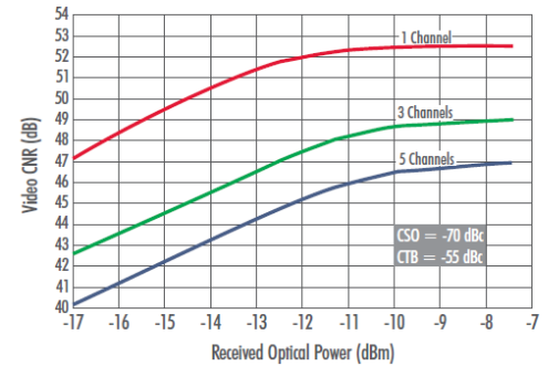
Carrier-to-Noise Performance
