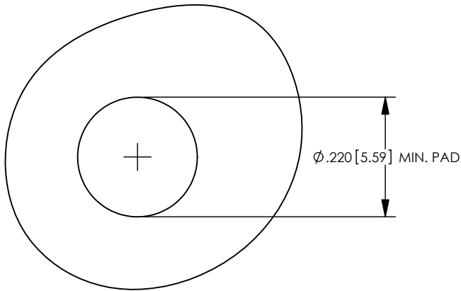
RECCOMENDED P.C. BOARD LAYOUT SCALE 4:1
