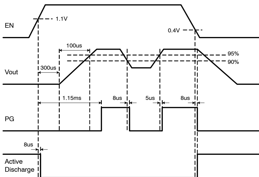
Figure 19. Power Good and Active Discharge Timing Diagram
